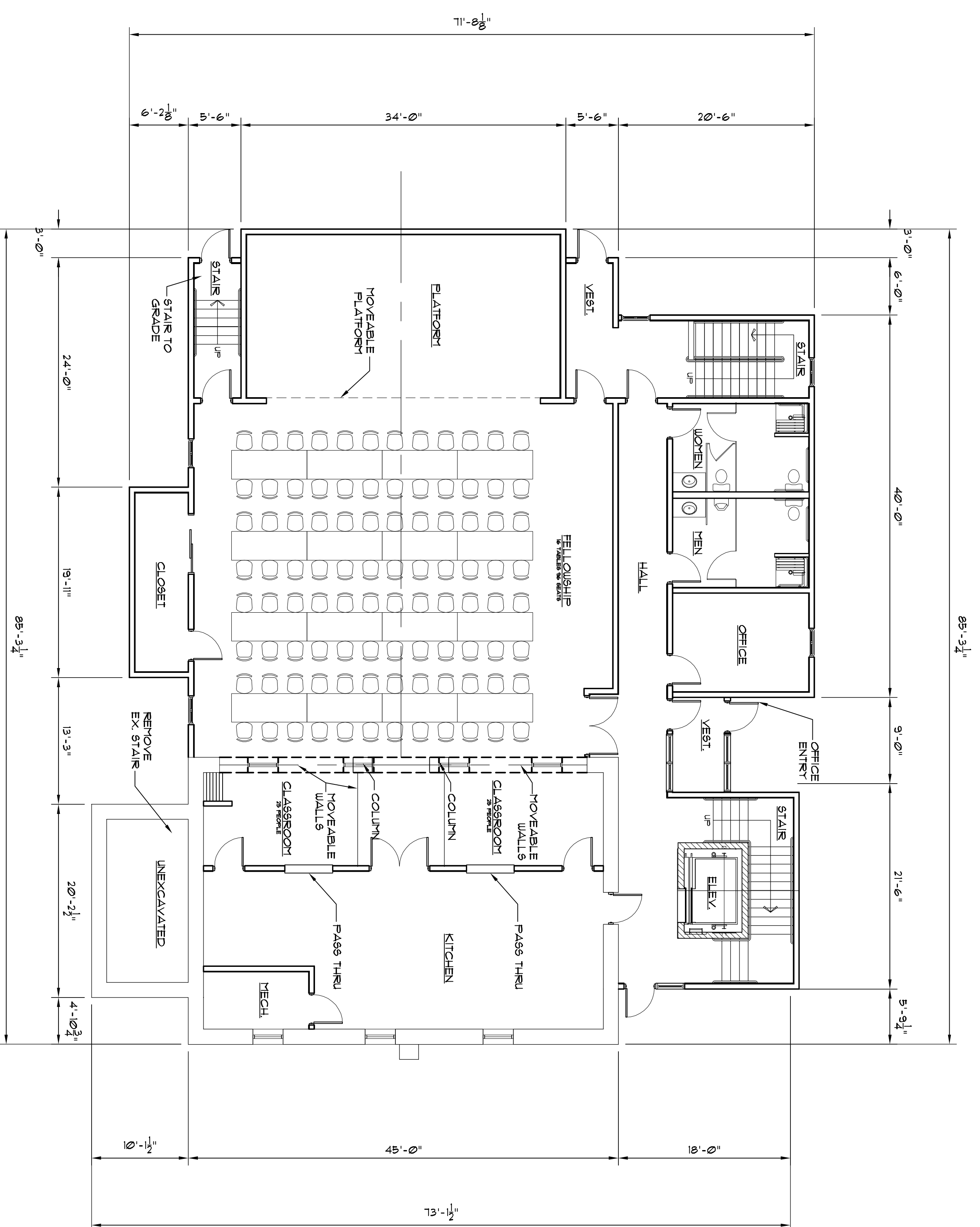
PROPOSED BASEMENT FLOOR PLAN SCALE: 1/8" = 1'-0"
