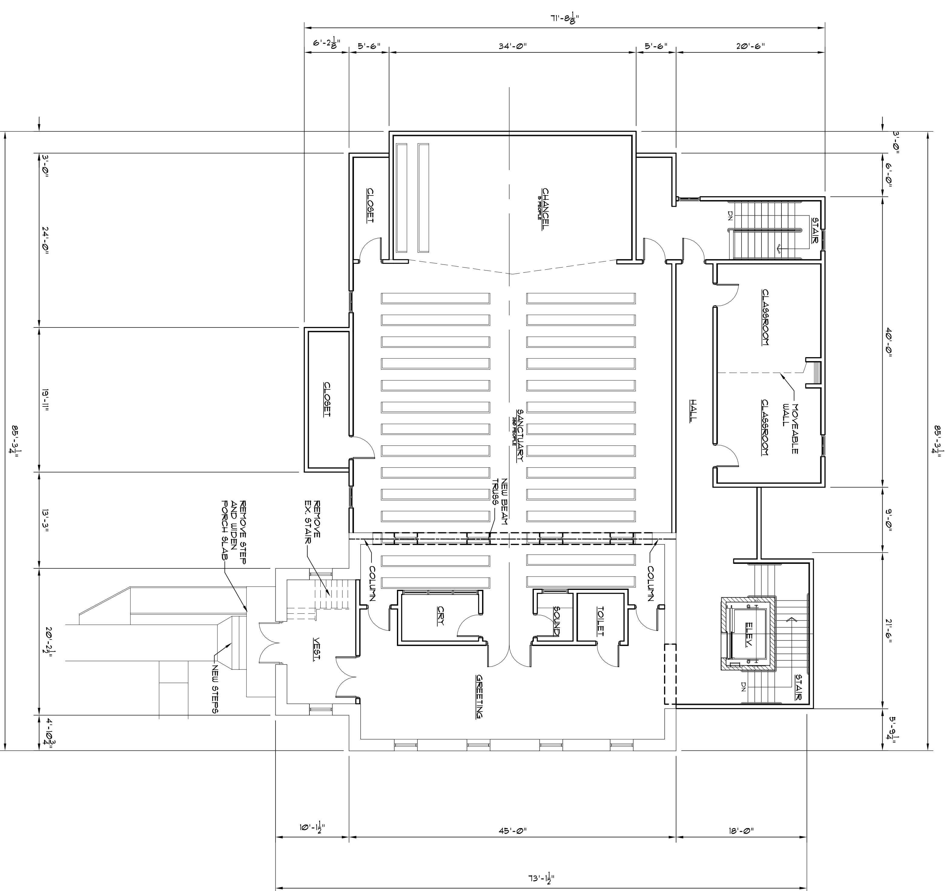
PROPOSED FIRST FLOOR PLAN SCALE: 1/8" = 1'-0"
